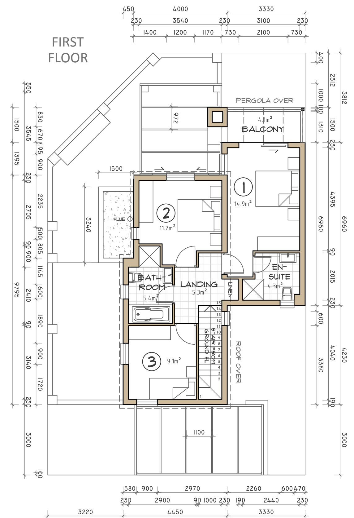
FLOOR PLANS 1:100 @ A3
